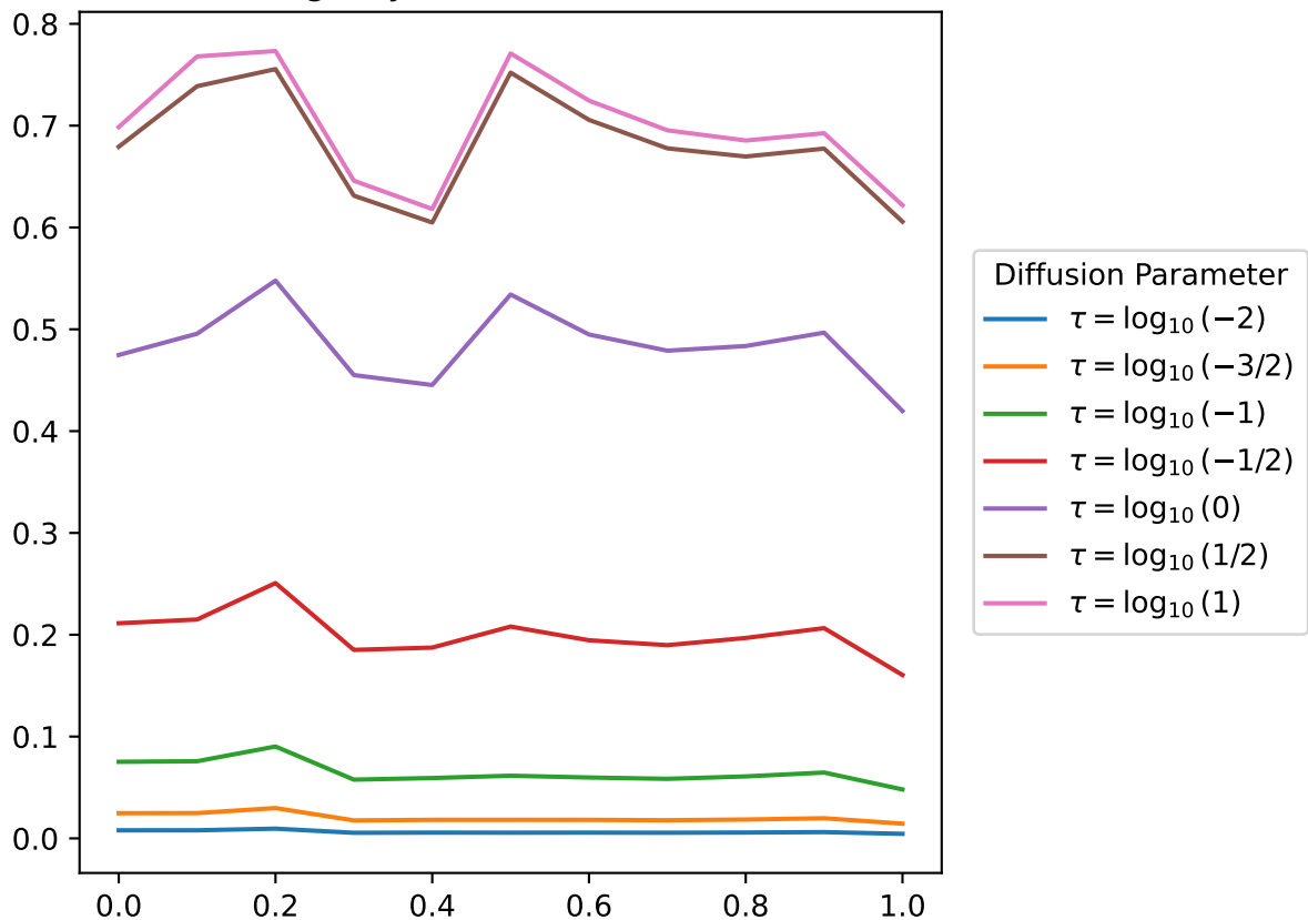
Average Dynamic Ricci Curvatures
